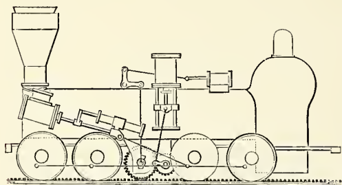
Fig. 9.—BALDWIN ENGINE FOR RACK-RAIL, 1847.
